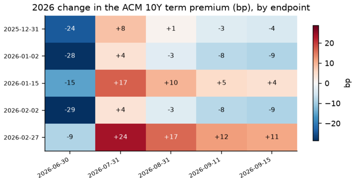
Figure 5. The 2026 change in the term premium, for 25 combinations of start and end date. Blue is negative, red is positive.
